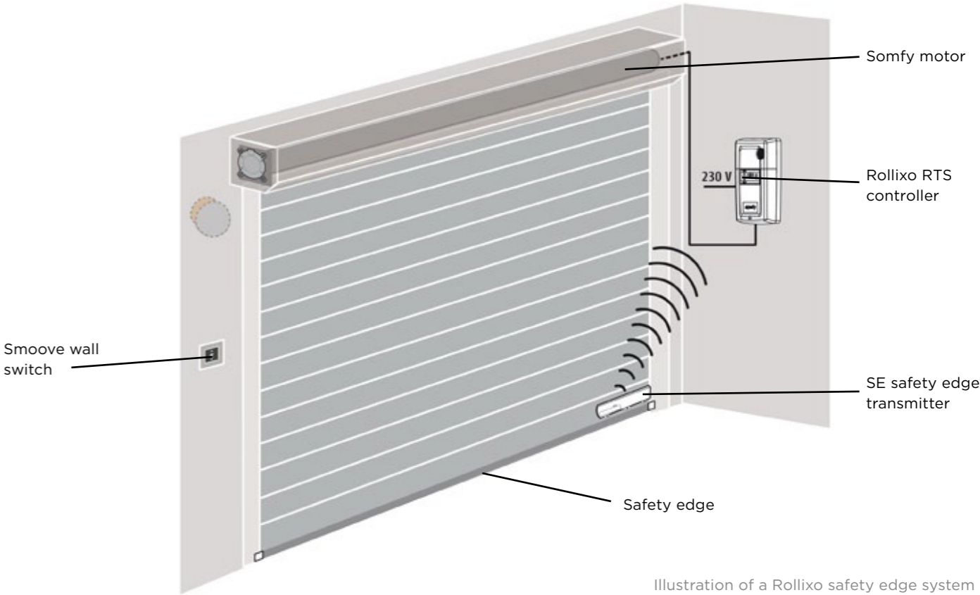
Illustration of a Rollixo safety edge system
